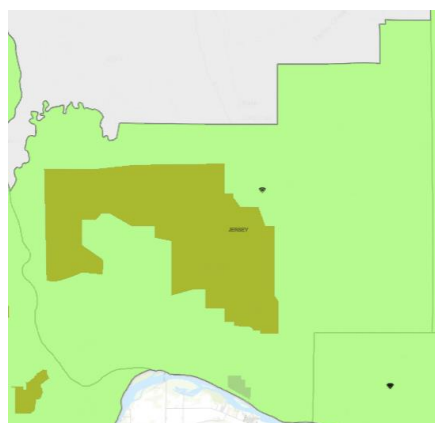
County Boundaries Connect Illinois Broadband Infrastructure Grants: 2,021 Accelerate Illinois Broadband Infrastructure Planning Program: Round 2, Round 1 Drive Up WiFi Hotspots Broadband Regional Engagement for Adoption + Digital Equity (READY) Grants: Round 2, Round 1 Illinois Connected Communities Grants: Round 2, Round 1
